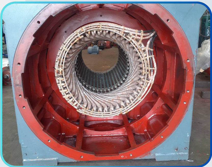
Rewinding HV & LV AC Motor DC Motor
